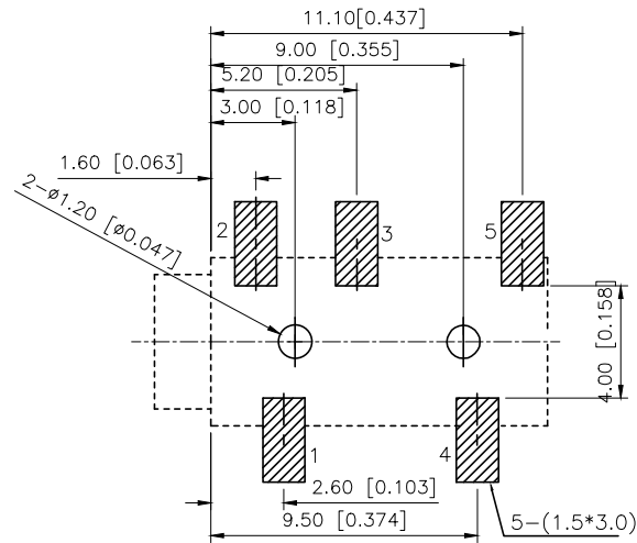
PCB LAYOUT TOP VIEW TOLERANCES:±0.05
