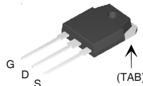
TO-3P (IXTQ)
