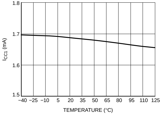
Figure 59. Internal IC Consumption, I CC1
