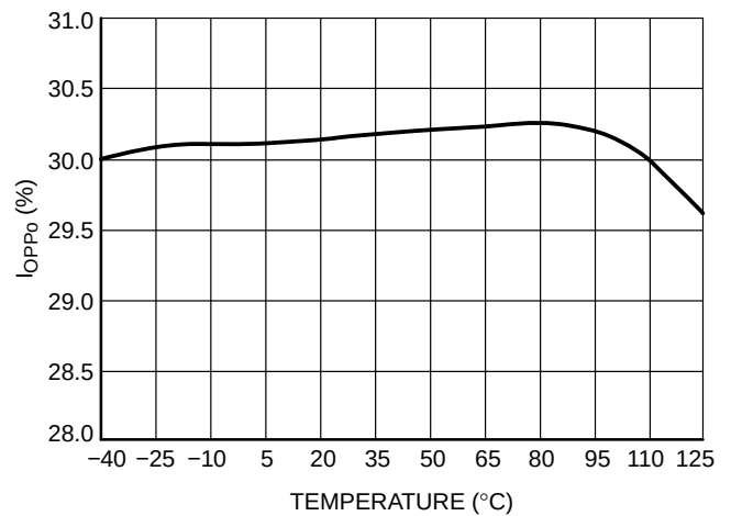
Figure 40. Set-point Decrease for OPP, I OPP0
