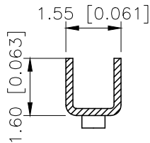
SECTION:C-C SCALE:1:1
