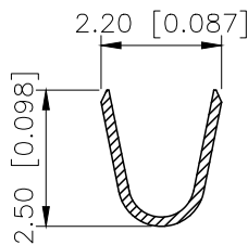
SECTION:A-A SCALE:1:1
