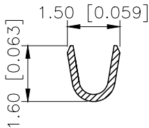
SECTION:B-B SCALE:1:1
