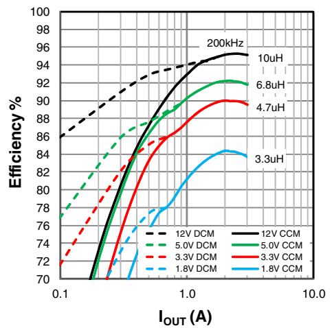
Figure 24: XR76203-Q efficiency, V_{\text{IN}}=24\text{V}
