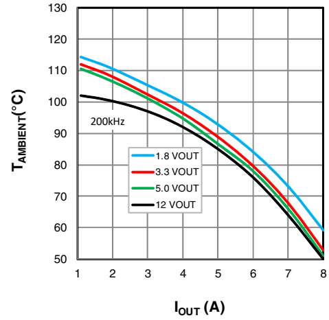
Figure 26: XR76208-Q, V_{IN}=24\text{V}
