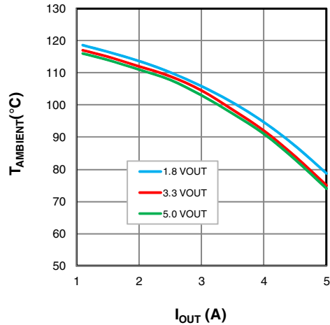
Figure 27: XR76205-Q, V_{IN}=12\text{V}
