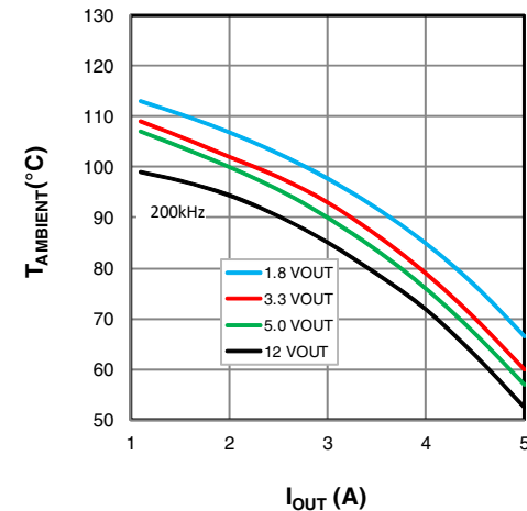
Figure 28: XR76205-Q, V_{IN}=24\text{V}
