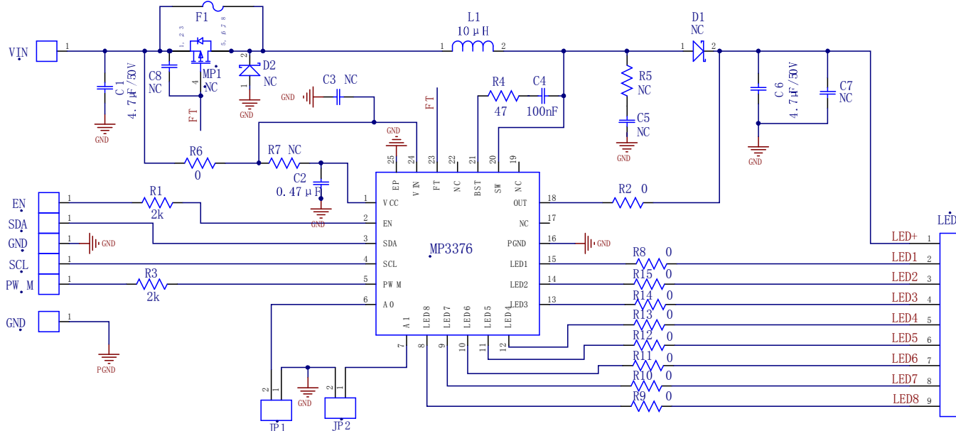
Figure 9: Typical Application Circuit
