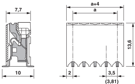
Dimensional drawing
