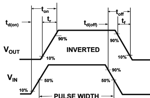
Figure 2: Switching Waveforms
