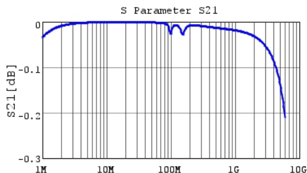
■ GRT21B5C1H183JA02 S21 DCOV, 25degC
