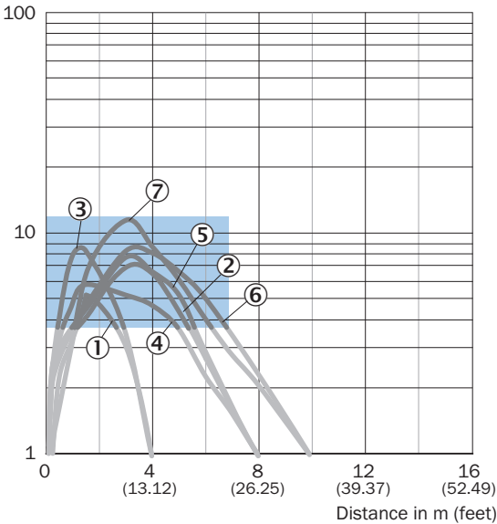
Operating reserve
