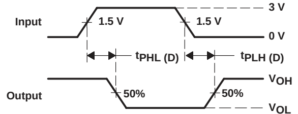
VOLTAGE WAVEFORMS
