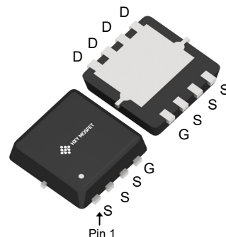
DFN3X3-8L (TSON-8(3.1x3.1))
