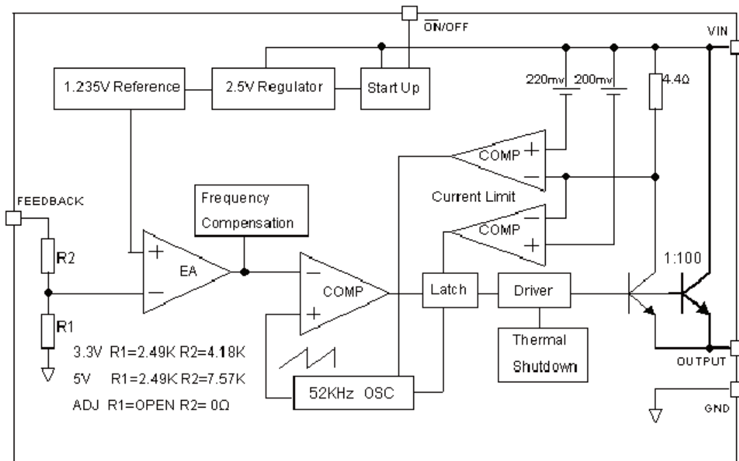
Functional Block Diagram of LM2576S-xx/NOPB
