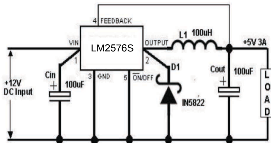
Typical Application of LM2576Sxx/NOPB
