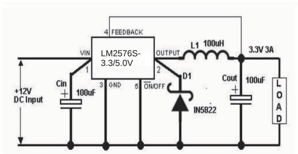
Figure 8. Typical Application of LM2576S For 3.3V, 5.0V
