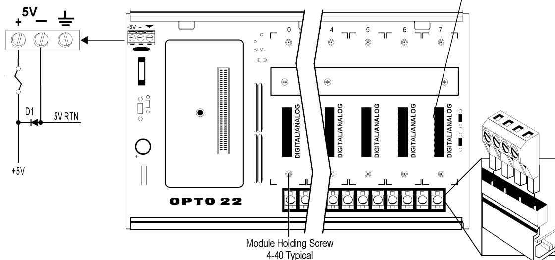
Power Schematic
