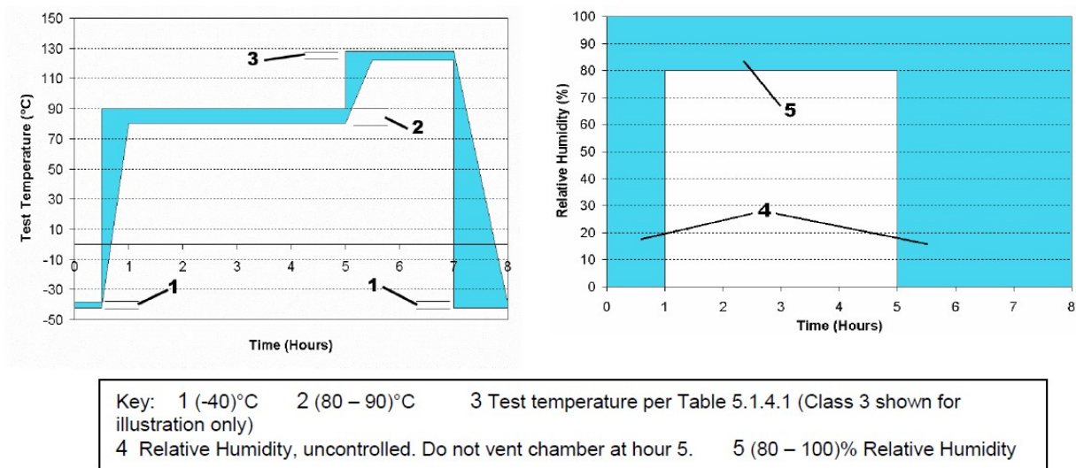
Fig 7. Temperature/humidity cycling schedule
