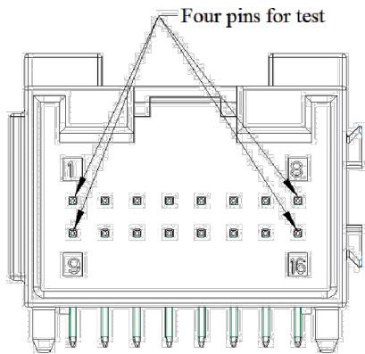
Fig 5. The positions of pins for current capability test
