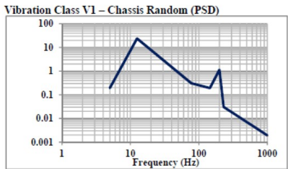
Fig 6. The vibration class V1 graphs
