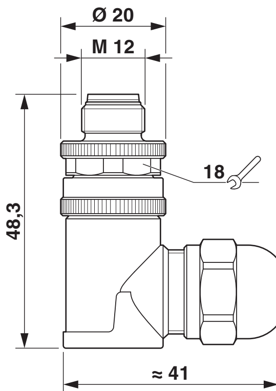
Dimensional drawing
