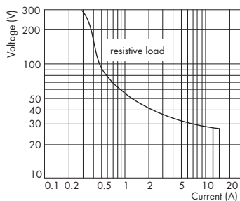
Load limit curve for 788-303 to 788-307, 788-506, 788-507 and 788-508
