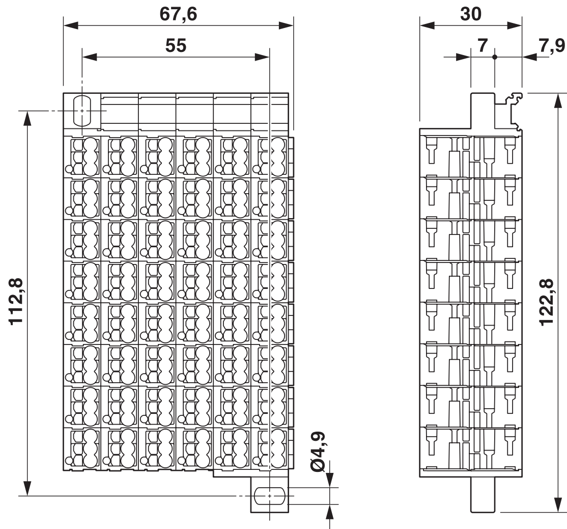
Dimensional drawing
