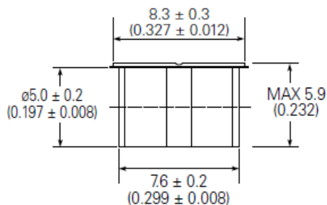
No Leads with -FT (GTCN35-XXM-R05-FT)
