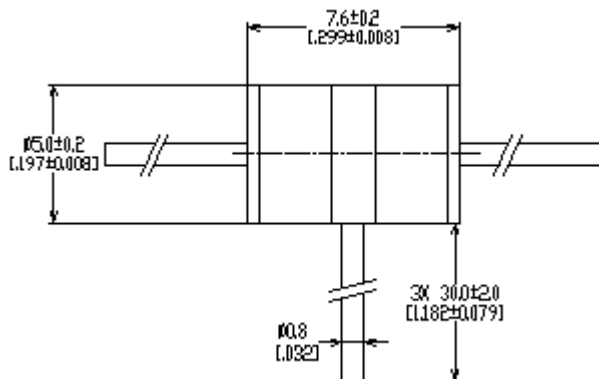
No Leads with -FT (GTCN35-XXM-R05-FT)
