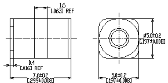
No Leads (GTCN35XXM-R05)
