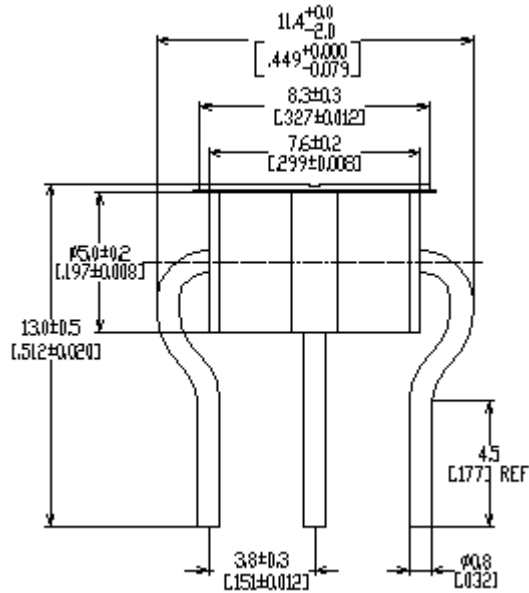
"T" Leaded (GTCT35-XXM-R05)
