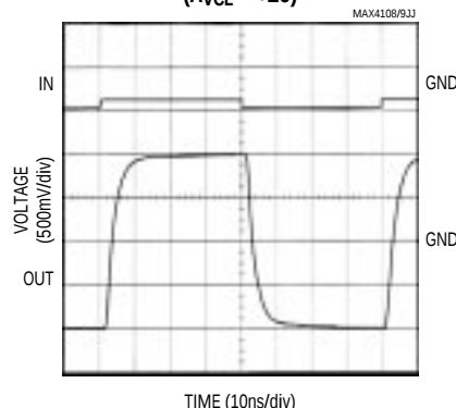
MAX4309 LARGE-SIGNAL PULSE RESPONSE ( A_{VCL} = +20 )
