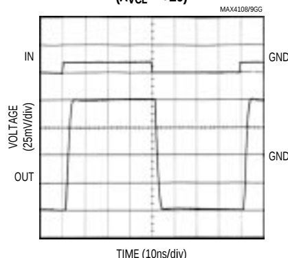
MAX4309 SMALL-SIGNAL PULSE RESPONSE ( A_{VCL} = +10 )
