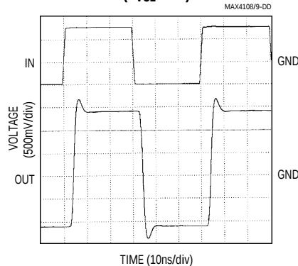
MAX4109 LARGE-SIGNAL PULSE RESPONSE ( A_{VCL} = +2 )
