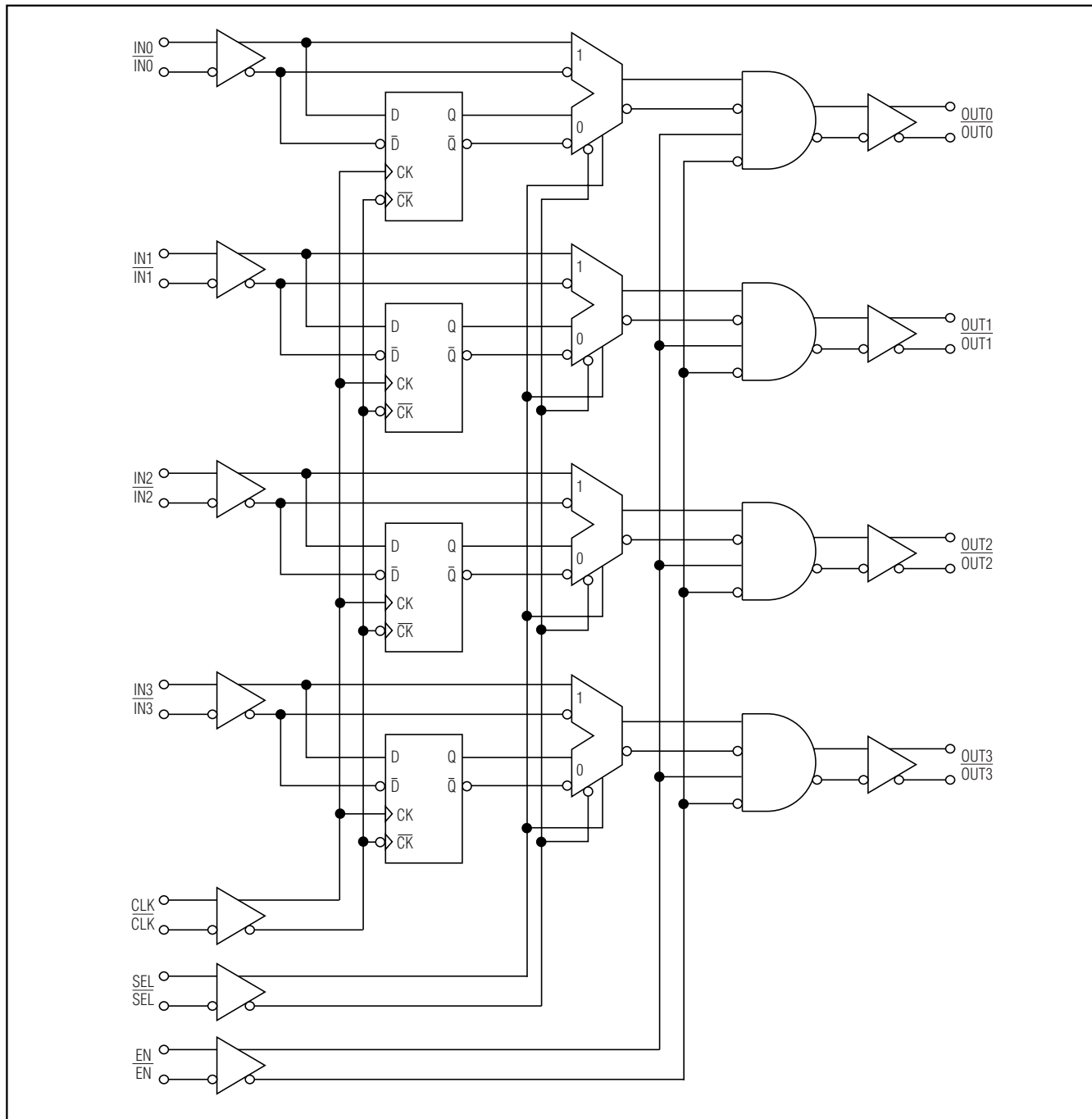
Functional Diagram
