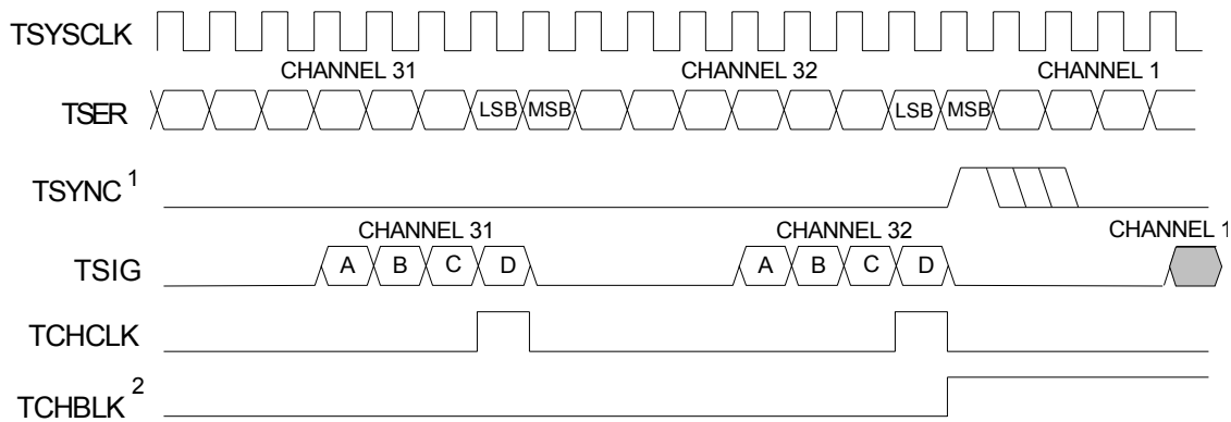
Figure 13-22. E1 Transmit-Side 2.048MHz Boundary Timing (Elastic Store Enabled)
