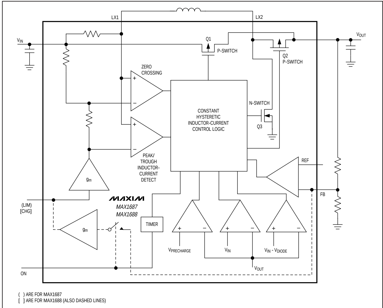
Figure 1. Functional Diagram
