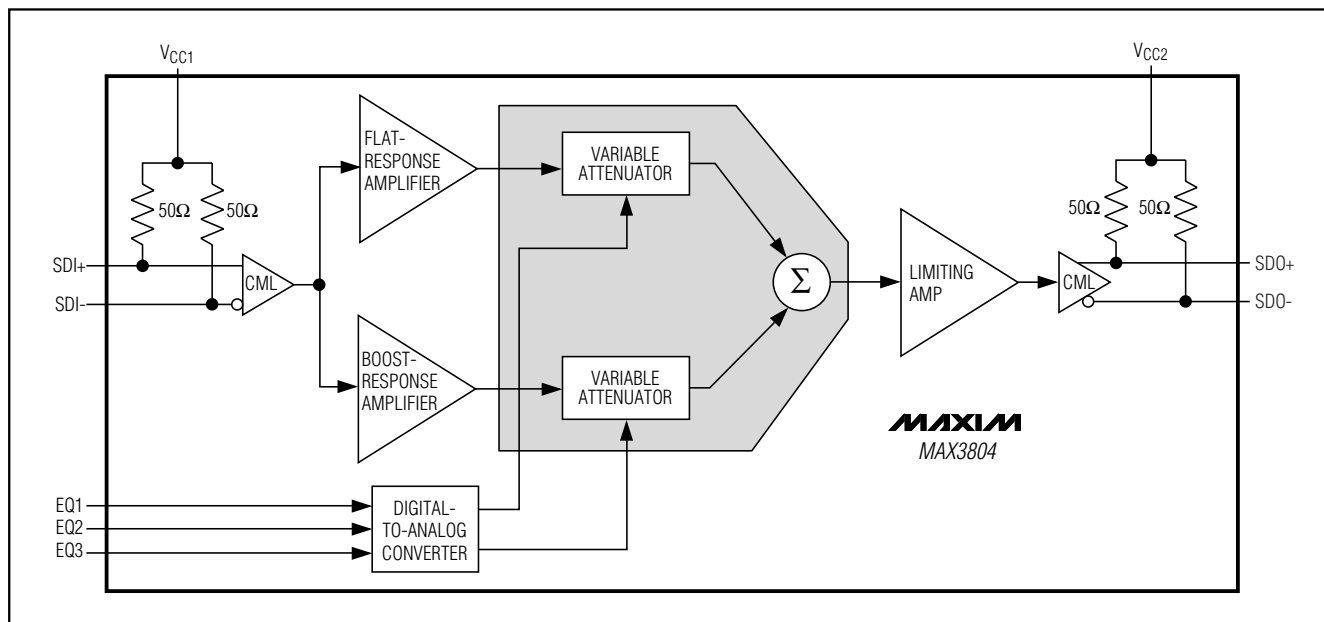
Figure 1. Functional Diagram
