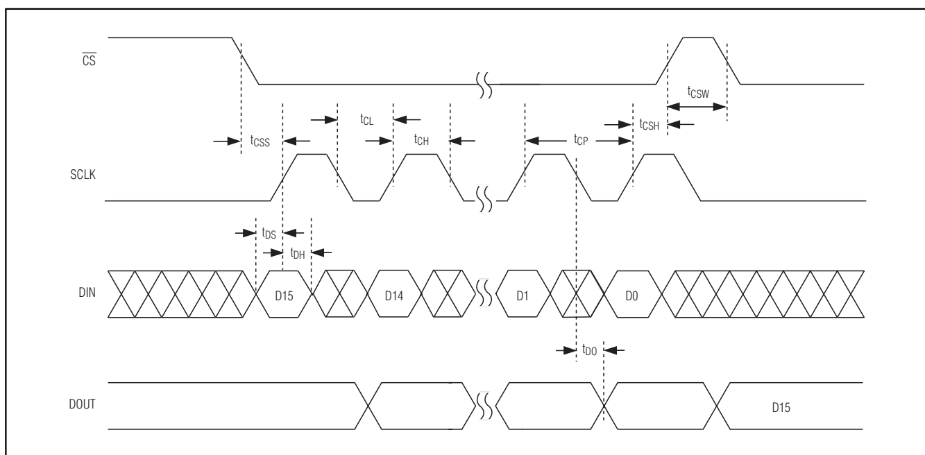
Figure 10. Timing Diagram
