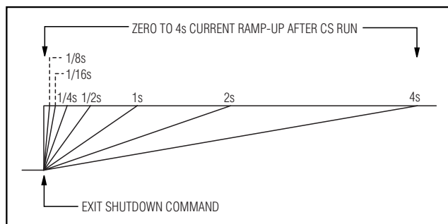
Figure 4. Ramp-Up Behavior
