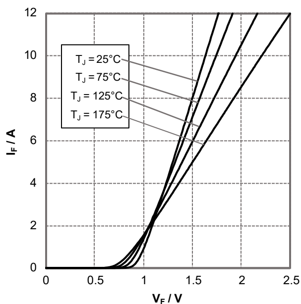
Figure 1. Forward Characteristics
