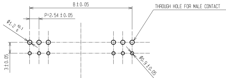
RECOMMENDED PC BOARD HOLE PATTERN
