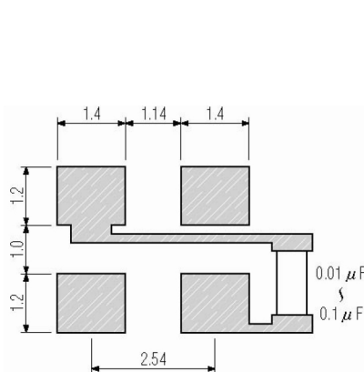
Figure 2) Suggested Land Pattern
