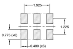
Figure 4) Top, Side, Bottom & Land
