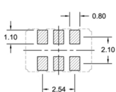
Figure 2) Top, Side, Bottom & Land
