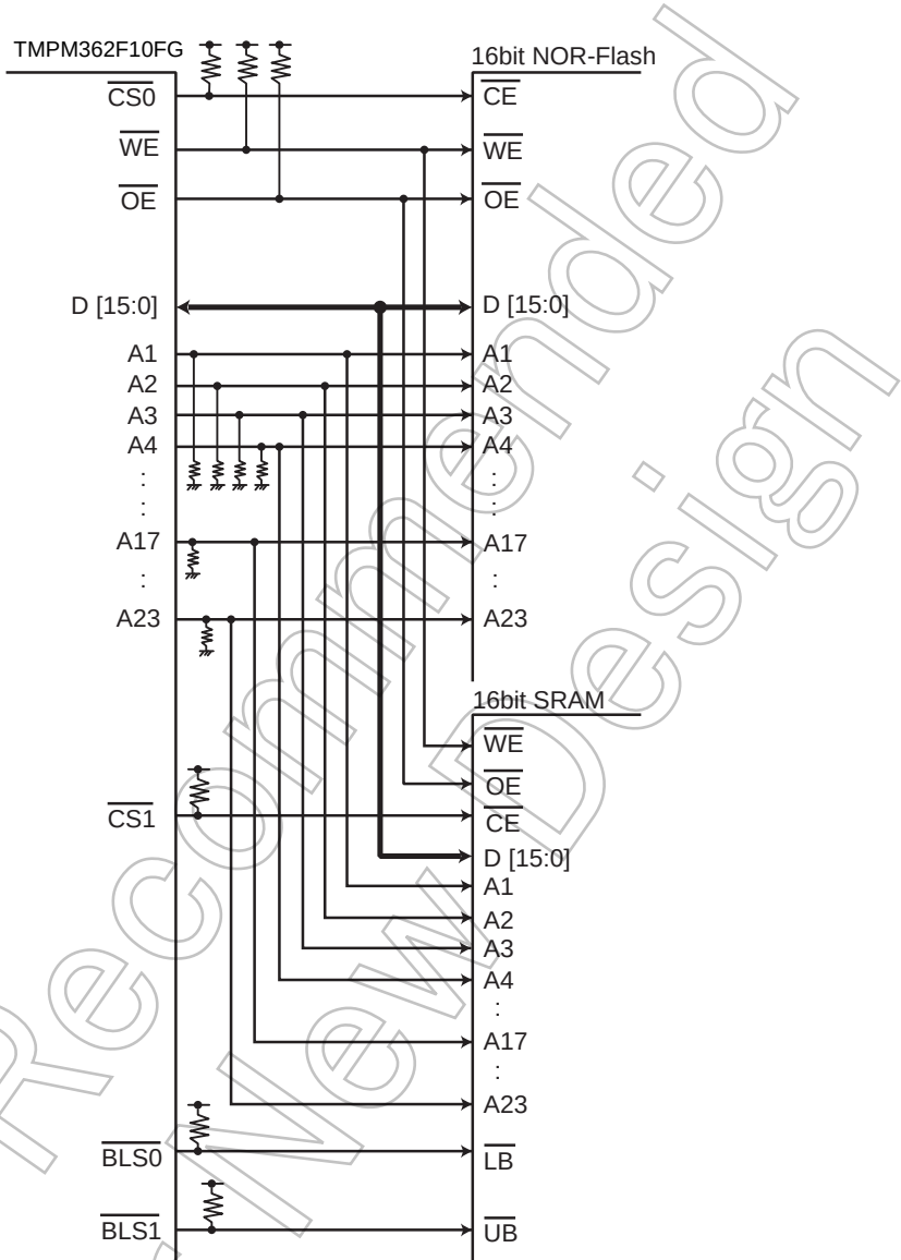
Figure 10-9 Connection Example for external 16bit SRAM and NOR-Flash (Separate mode)
