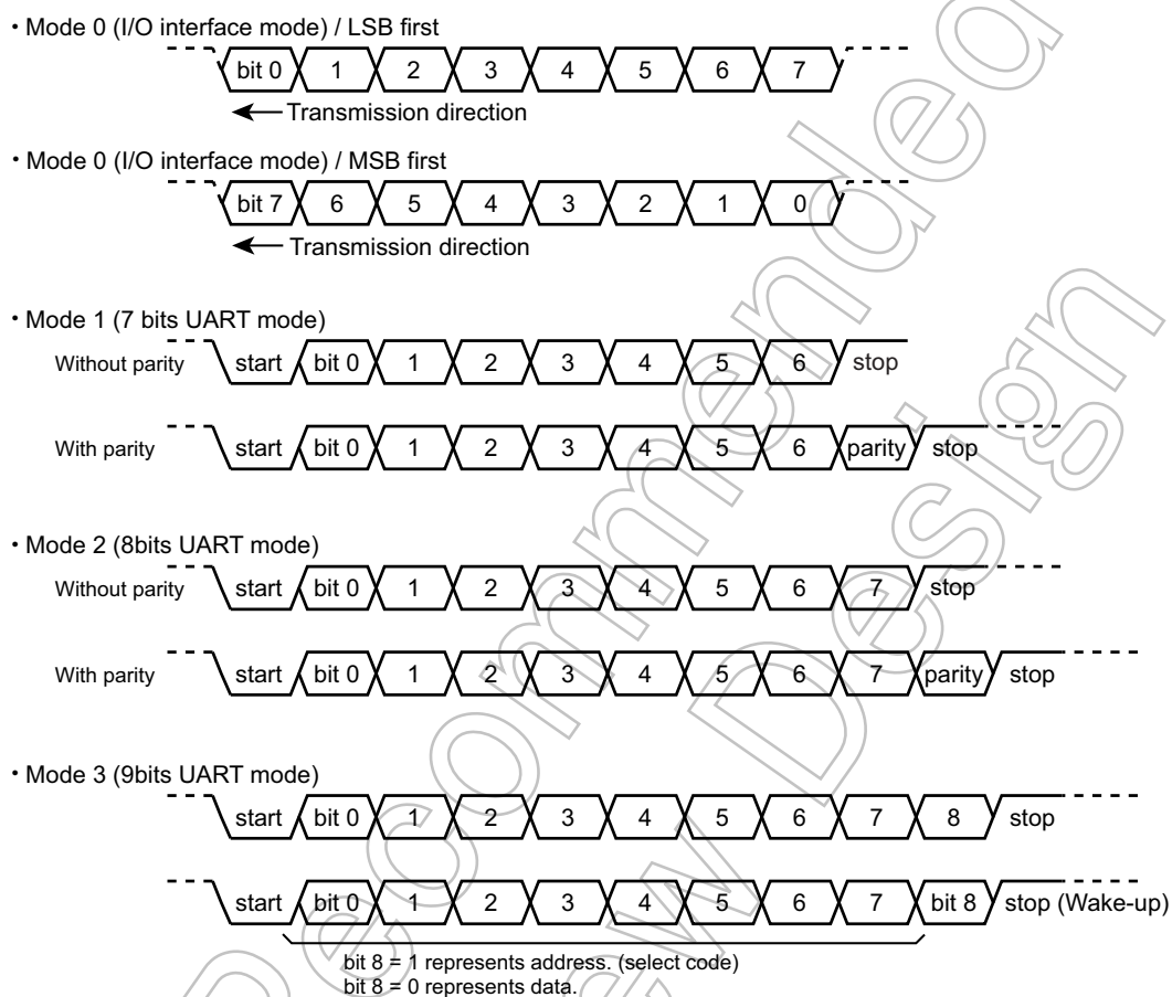
Figure 12-2 Data Format
