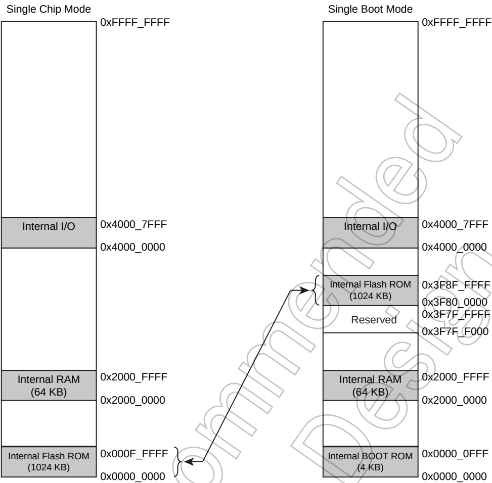
Figure 22-3 Memory Maps for TMPM362F10FG
