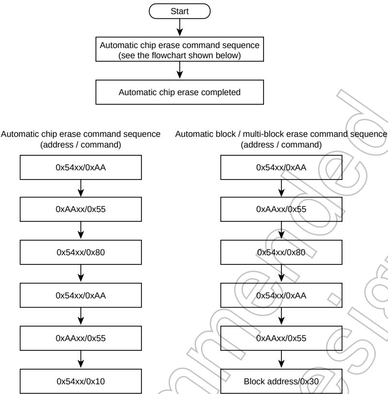
Figure 22-11 Automatic Erase
