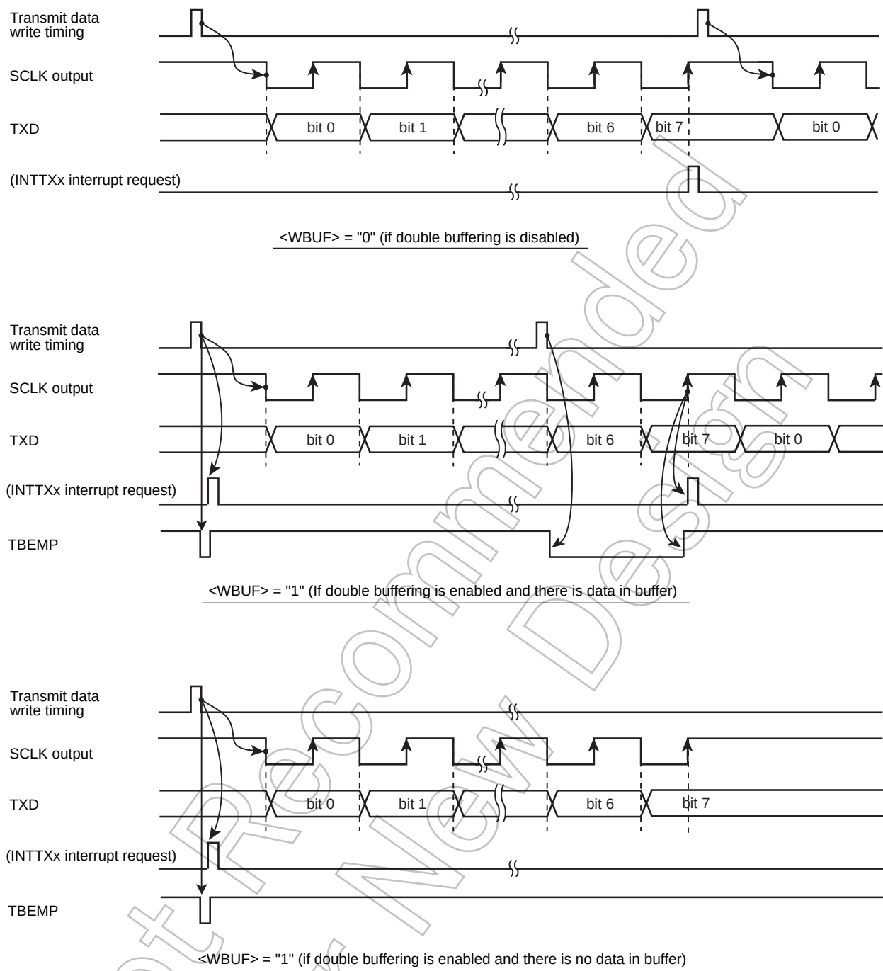
Figure 12-12 Transmit Operation in the I/O Interface Mode (SCLK Output Mode)
