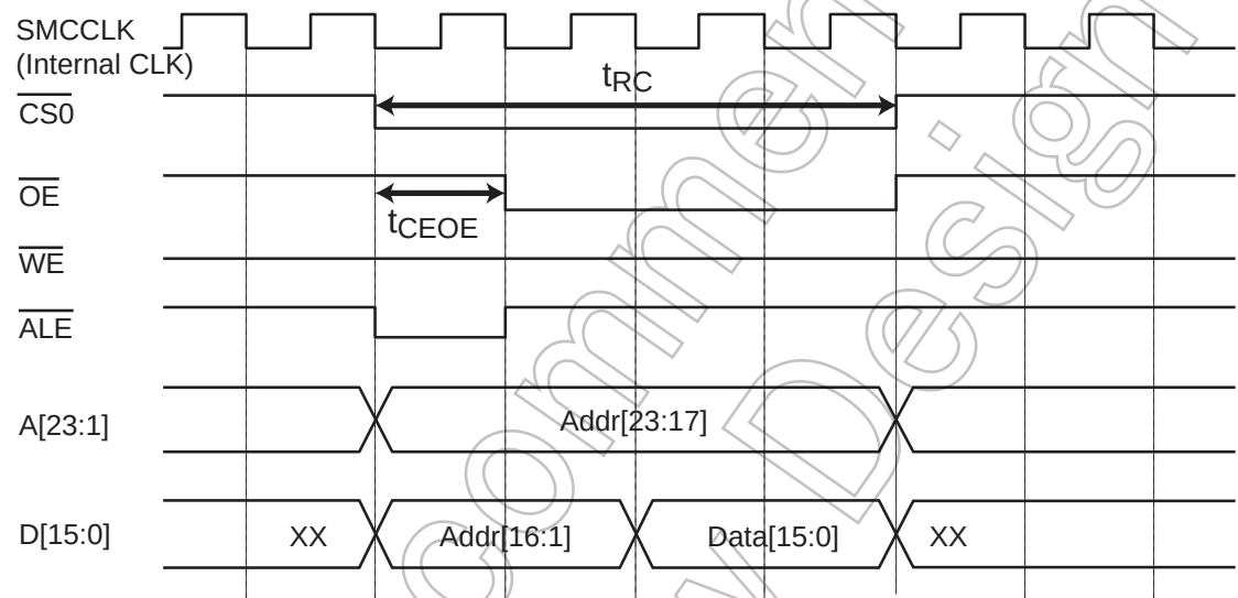
Figure 10-6 Asynchronous Read
