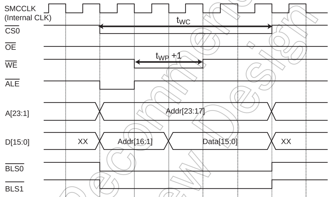
Figure 10-7 Asynchronous Write
