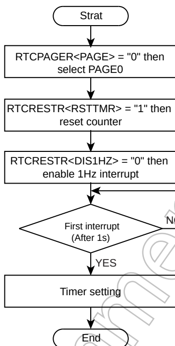
Figure 21-3 Flowchart of the clock data writing
