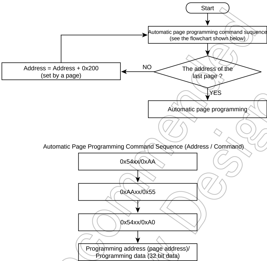
Figure 22-10 Automatic Programming
