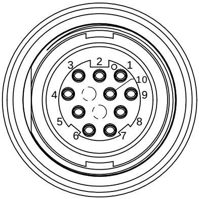
FACE VIEW W4291-10SG-3ES 10-POS.
