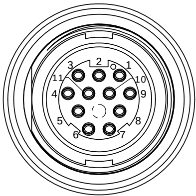
FACE VIEW W4291-11SG-3ES 11-POS.
