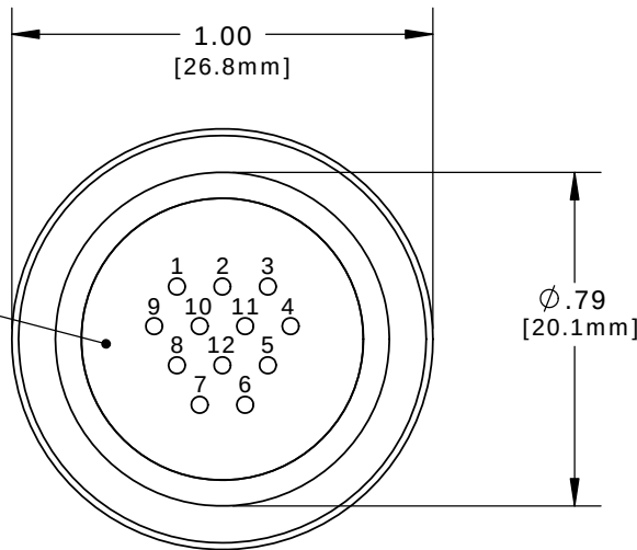
PC TAIL VIEW W4291-10SG-3ES - 10-POS. (11&12 CLOSED) W4291-11SG-3ES - 11-POS. (12 CLOSED) W4291-12SG-3ES - 12-POS. (ALL OPEN)
