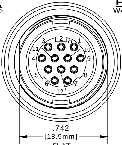
FACE VIEW W4291-12SG-3ES 12-POS.
