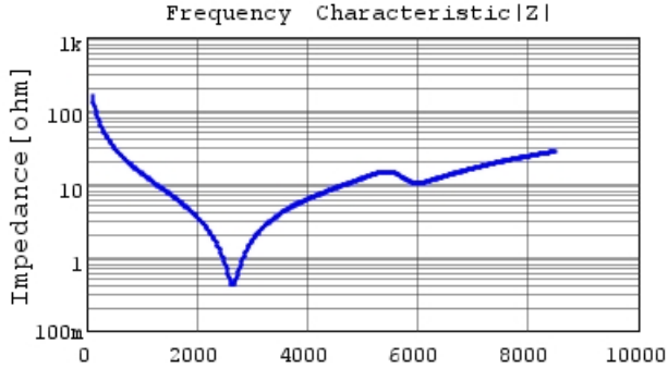
■ GRT1555C1E100JA02 |Z| DCOV,25degC
