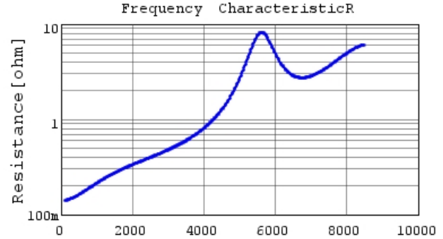
■ GRT1555C1E100JA02 R DCOV,25degC
