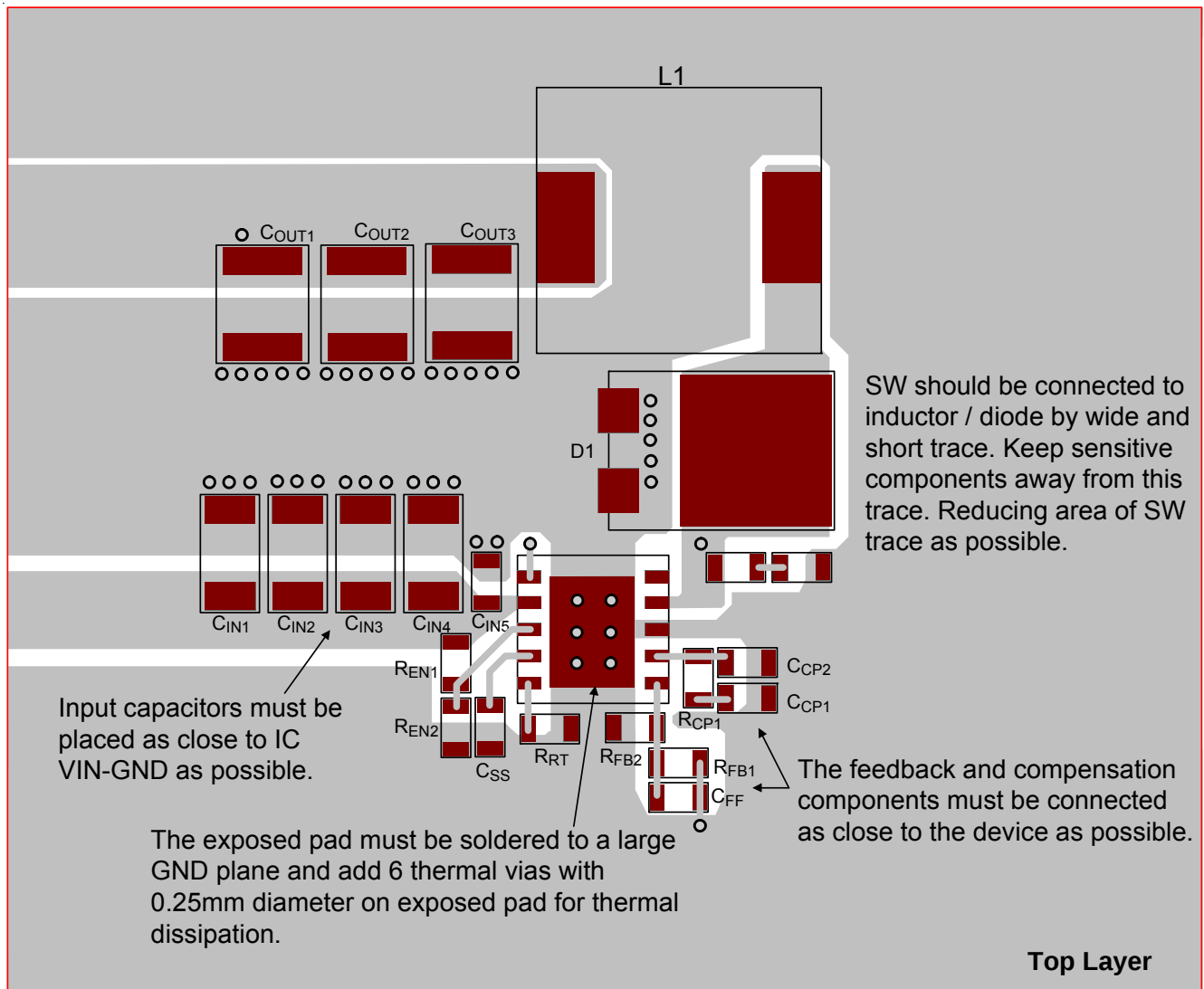
Figure 16. Layout Guide for RTQ6363GQW (Top Layer)
