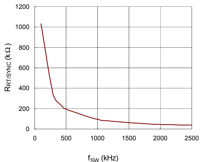
Figure 3. Switching Frequency vs. R_{RT/SYNC}
