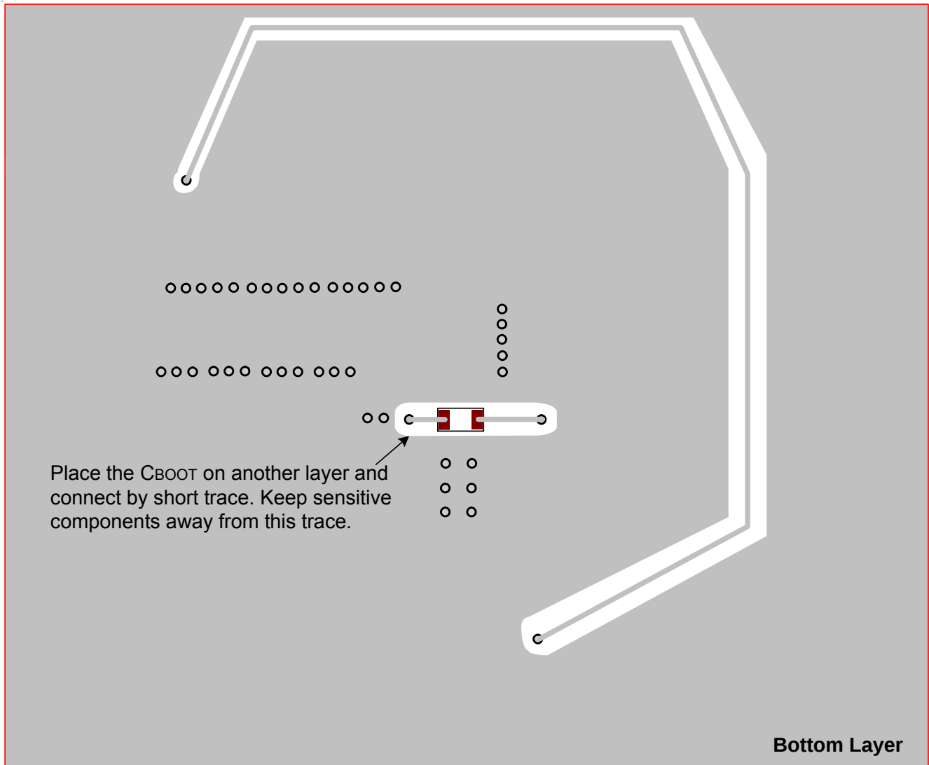
Figure 17. Layout Guide for RTQ6363GQW (Bottom Layer)
