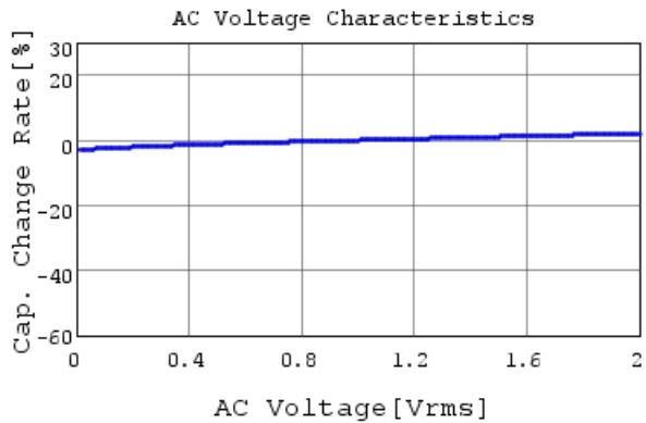
GRM319R71H104JA01 C-AC Voltage capchange, Dc
