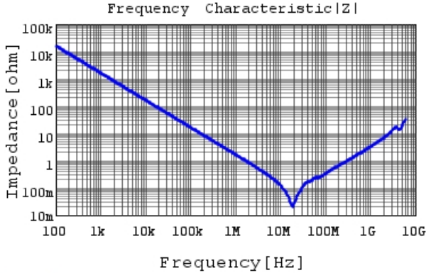
GRM319R71H104JA01 |Z| DCOV,25degC
