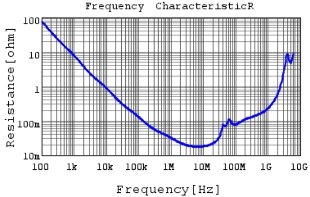
GRM319R71H104JA01 R DCOV,25degC
