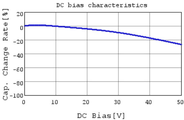
GRM319R71H104JA01 C-DC bias capchange, 25.0C
