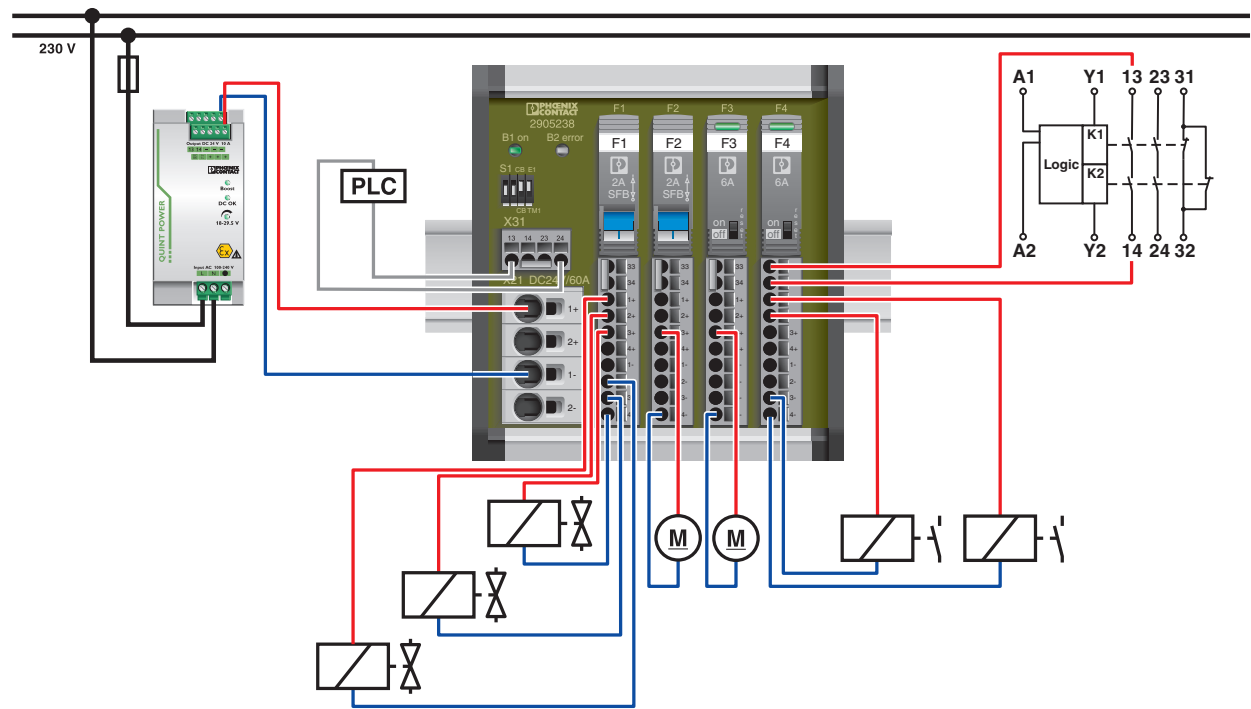
Application drawing
