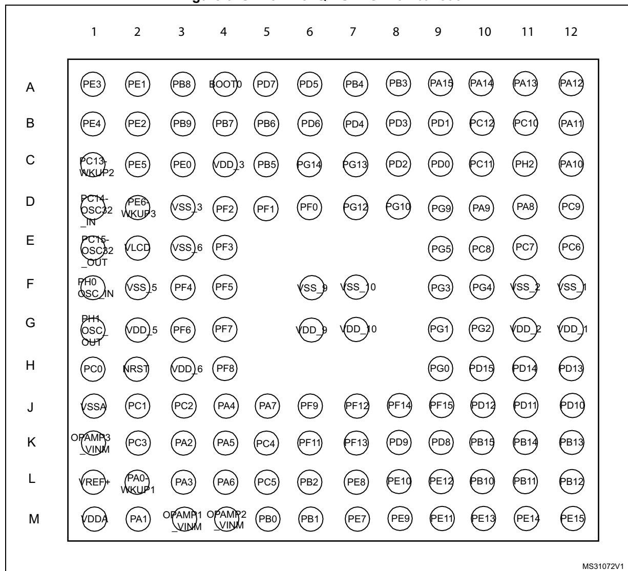
Figure 6. STM32L15xQD UFBGA132 ballout
