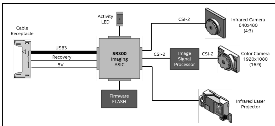
Figure 4-1: Embedded 3D Imaging System
