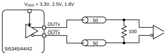
DC Coupled LVDS
