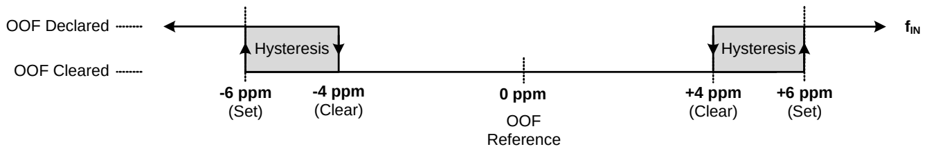
Figure 15. Example of Precise OOF Monitor Assertion and De-assertion Triggers
