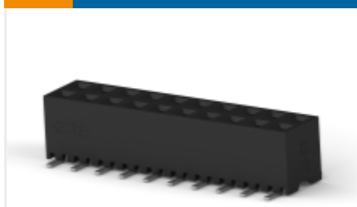
TE Part #3-2307819-0 30P,2MM,BB,REC,DRV,T,SMD,AU.76, TR,W/CP
