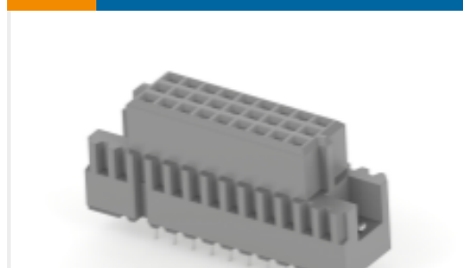
TE Part #5-1571437-1 27P TR VERT RCPT ASSY,EUROCARD
