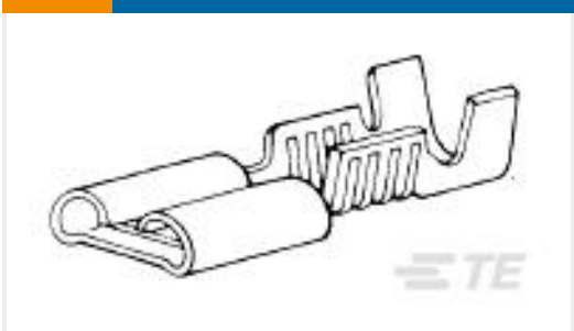
TE Part #60214-2 187 FASTON REC 20-16 AWG TPBR
