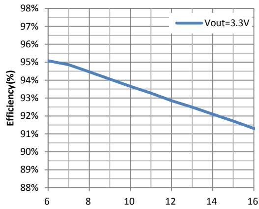
Efficiency vs. Vin Iout=1A
