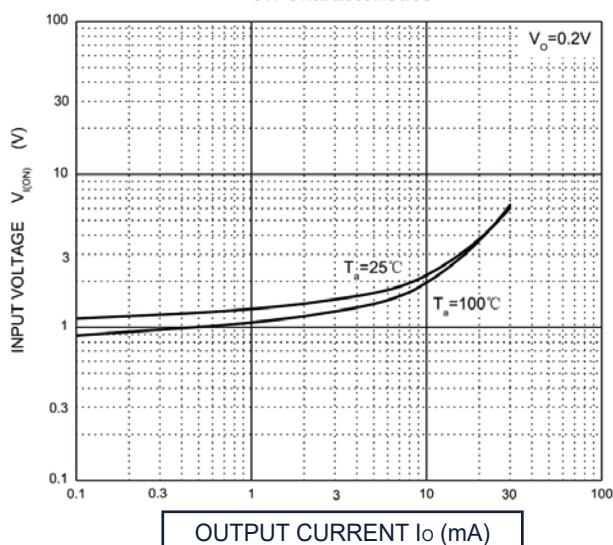
ON Characteristics
