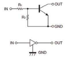
Equivalent Circuit
