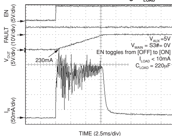
AUX Inrush Current into Large C_{\text{LOAD}}
