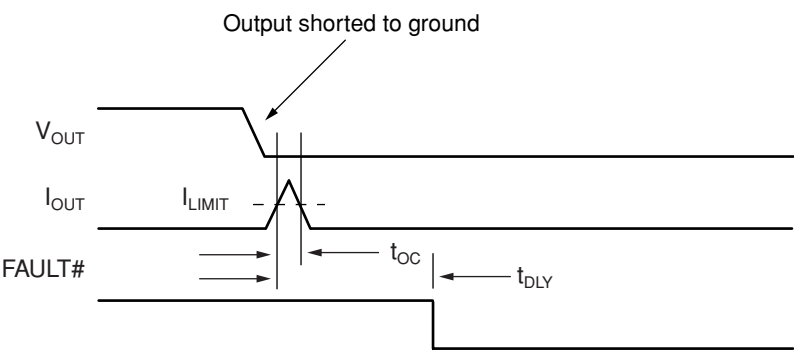
Figure 4. Overcurrent Response Timing
