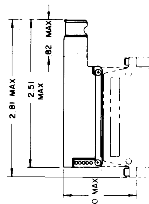
1 INCH RECEPTACLE ASSY INSTALLATION DATA REF
