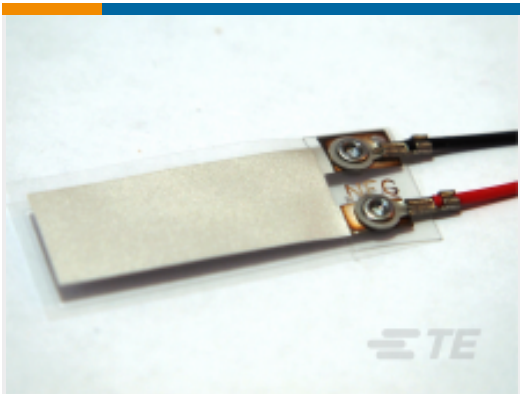
TE Part #11028414-00 Piezoelectric Vibration Sensor, Polymer
