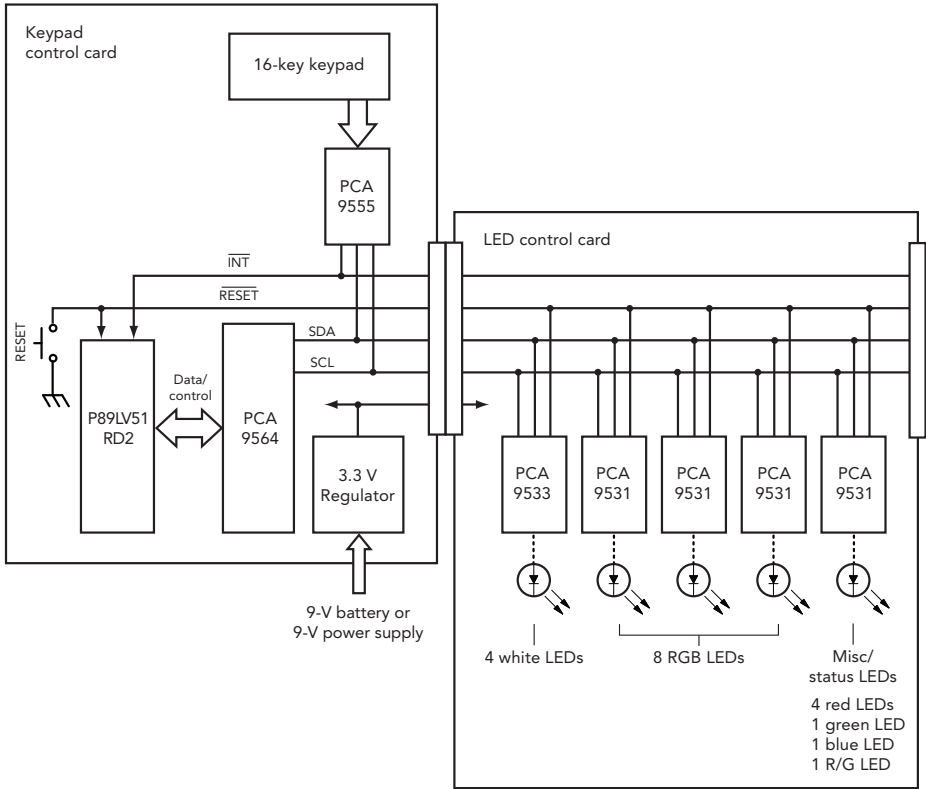
Block diagram of demo board
