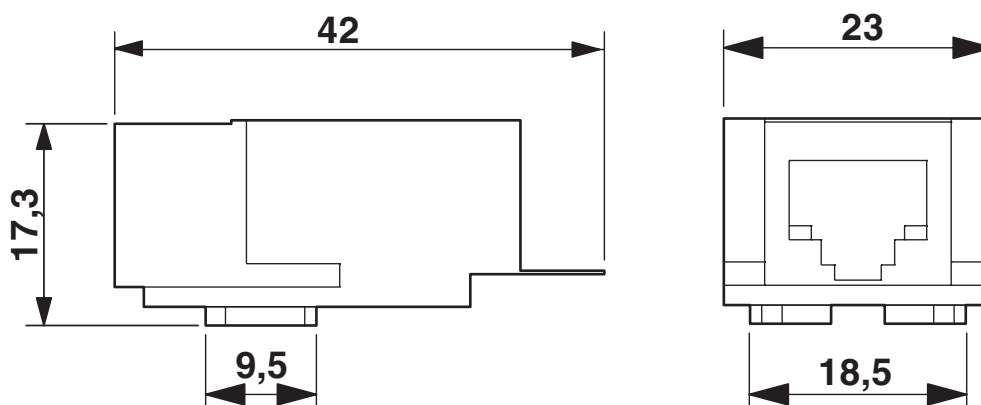
Dimensional drawing
