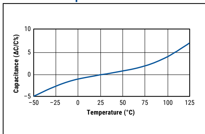
Typical Capacitance vs. Temperature at 1 kHz
