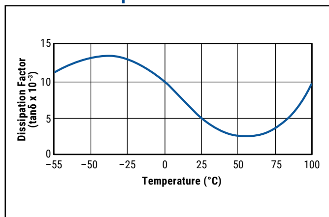
Typical Dissipation Factor vs. Temperature at 1 kHz
