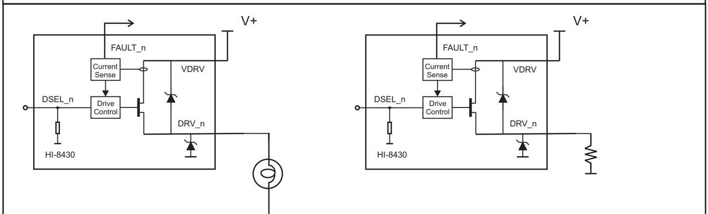
Figure 10 Highside Output Driving Resistive Load
