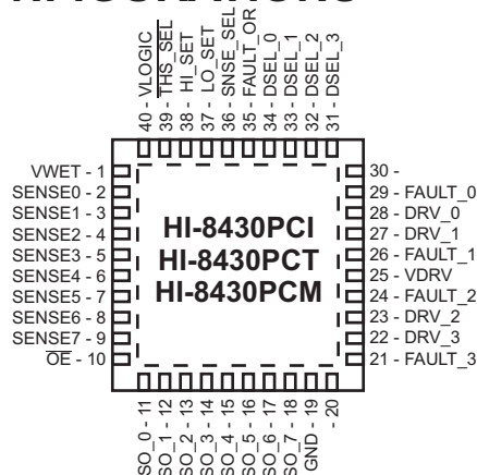
40 Pin Plastic 6mm x 6mm Chip-scale package
