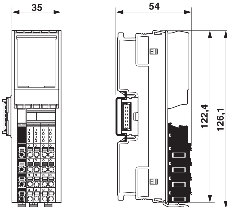
Dimensional drawing
